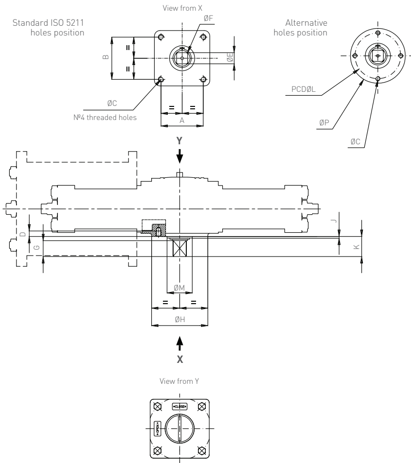
Actuator shown in closed position
