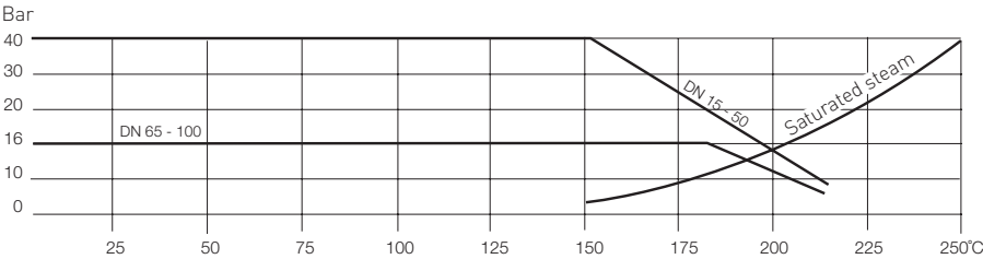
OPERATING PRESSURE AND TEMPERATURE FOR STANDARD SEALS* CAPRO 327/627 SERIES II
