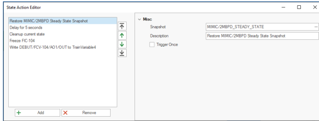
The State Action Editor.
