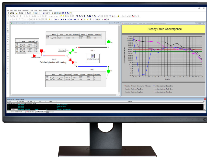
Figure 3: Track simulated batch movements with the Steady State Convergence chart. Current pipeline activities are shown in the events and alarms pane.
