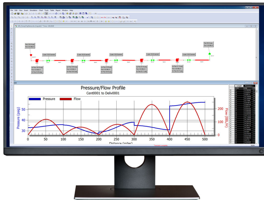
Figure 5: Monitor flow and pressure constraints with easy to understand charts.
