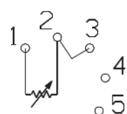
带补偿回路的热电阻 (2)
